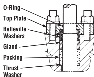
Triple Seal PTFE Cup and Cone
