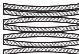
Triple Seal Belleville Washer Arrangement
